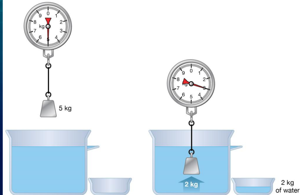
Archimedes' principle
